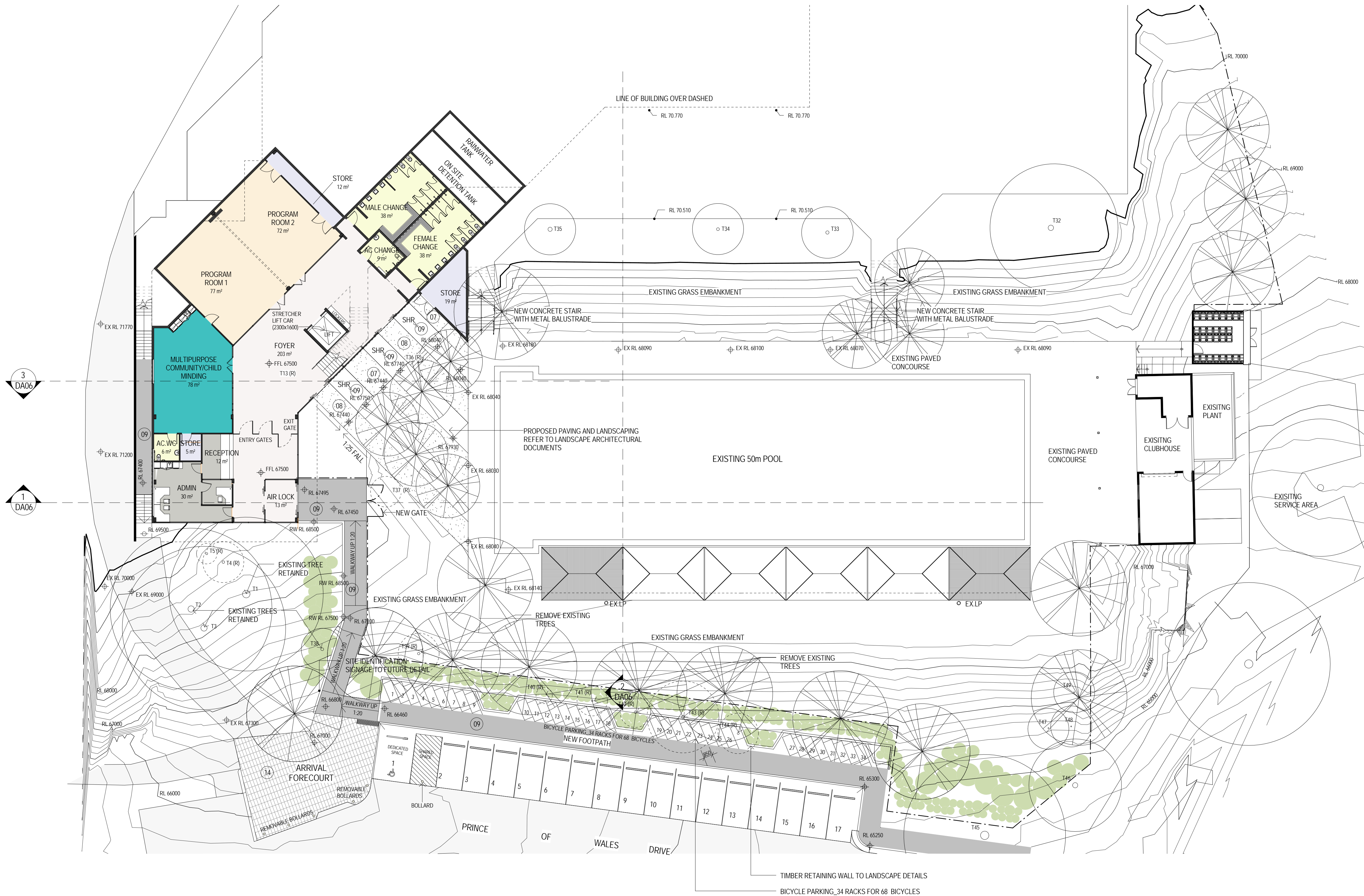
LOWER GROUND FLOOR PLAN 1:200
